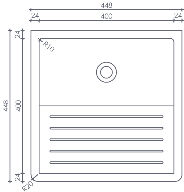
VISTA FRONTAL
